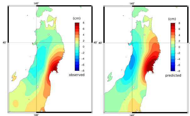
Vertical velocities
